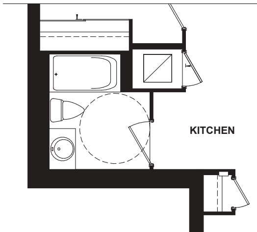
PARTIAL BARRIER-FREE PLAN (FLOORS 3 - 16, 23-PENTHOUSE)
